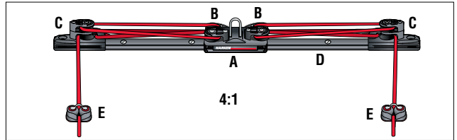
4:1 Remote Cleat: If the traveler is mounted ahead of the companionway, place the cleats at the aft-edge of the cabin house.
