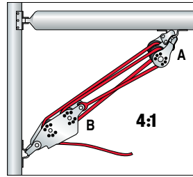
4:1 V-Jam: This simple 4:1 self-cleaning vang is used on small dinghies.
