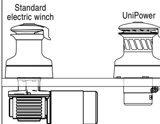
Low-profile electric motor saves headspace.
