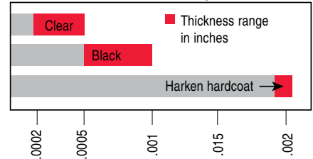
6061-T6 Aluminum Anodizing Thickness
