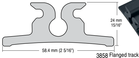
3858 Flanged track
