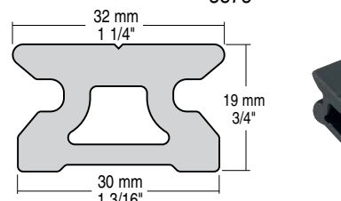
R32 Big Boat traveler track
