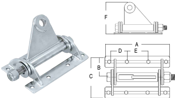
PIVOTING MAST FITTINGS
