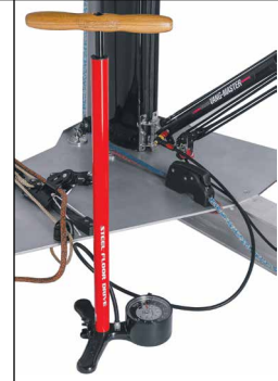
Lezyne stand-up and hand-held pumps fit naturally to the Vang-Master Schrader valve, helping adjust boom height and resistance level.
