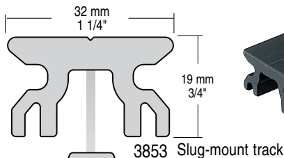
3853 Slug-mount track
