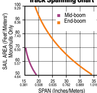
13 mm High-Beam Track Spanning Chart
