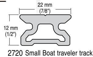
2720 Small Boat traveler track
