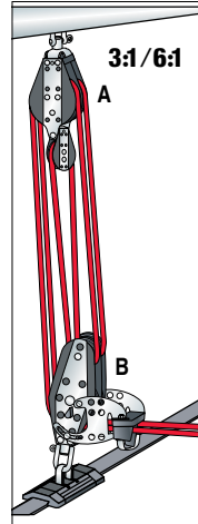
3:1/6:1: This 3:1/6:1 two-speed system is used on end-boom sheeting and mainsails up to 22.3 m 2 (240 ft 2 ).
