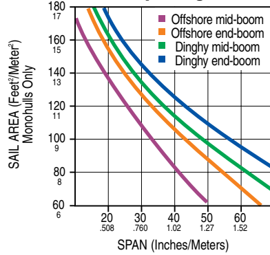
22 mm High-Beam Track Spanning Chart
